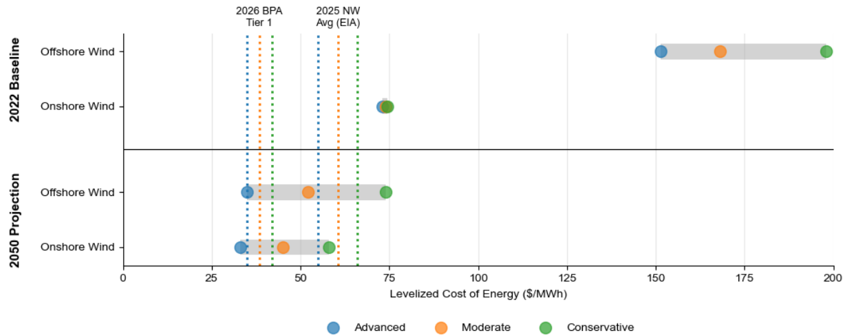
Figure 74: Offshore and Onshore Wind vs BPA Tier 1 2 and NW Average (2025) LCOE 3
