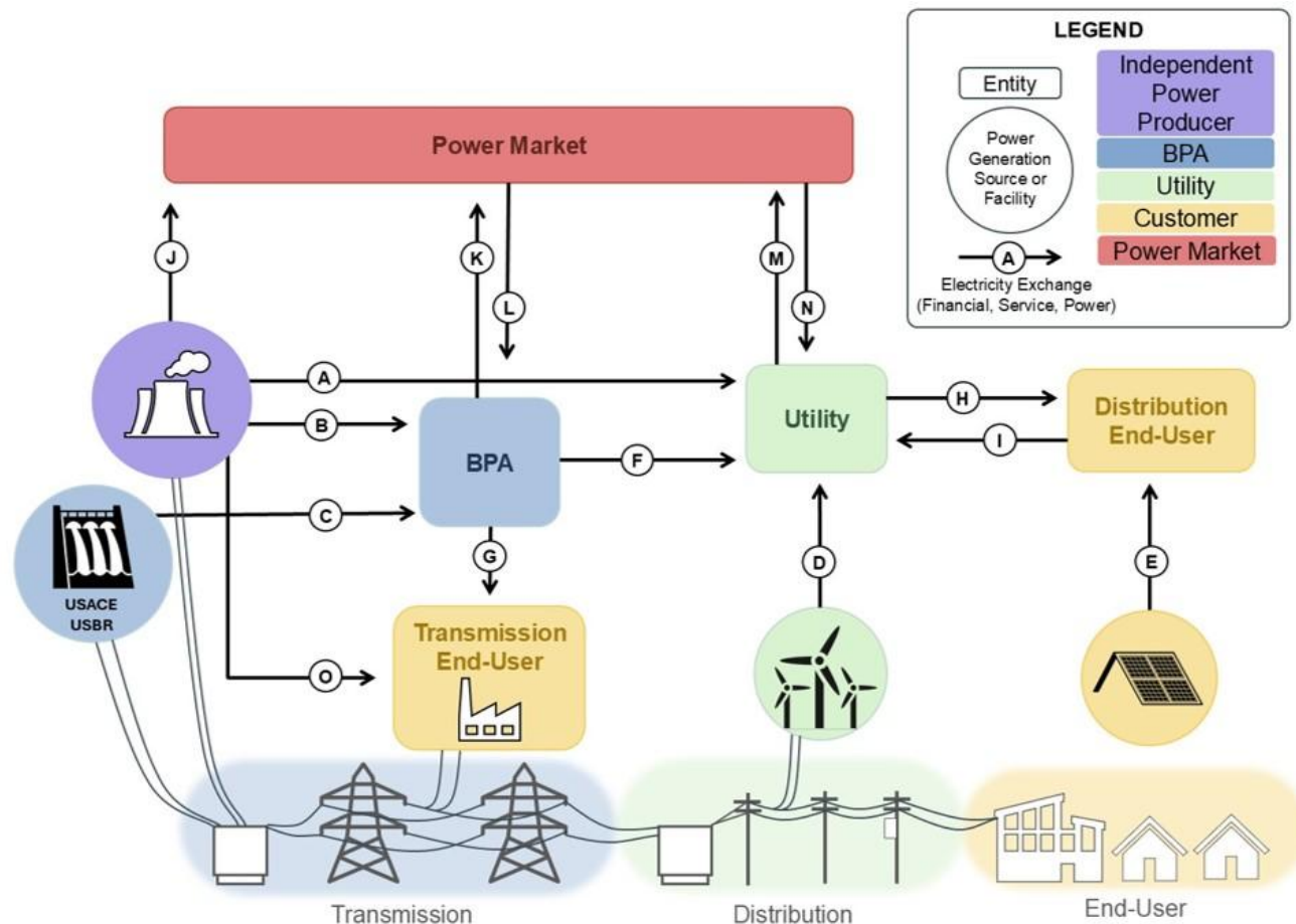
Figure 17: Northwest Electricity Exchange
